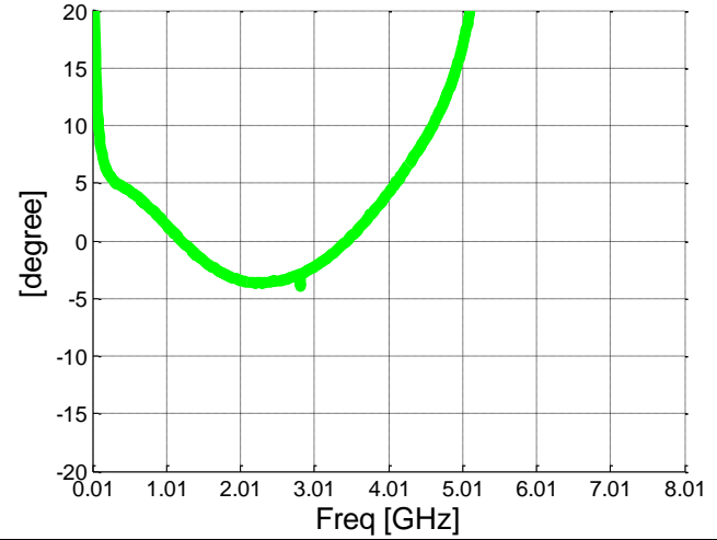
Phase balance
