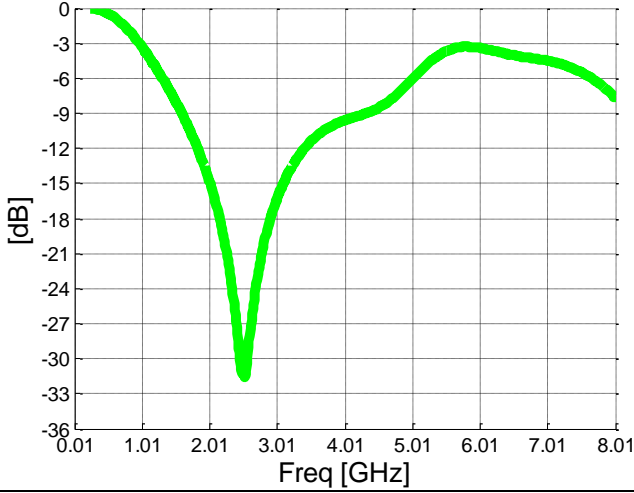
Return Loss
